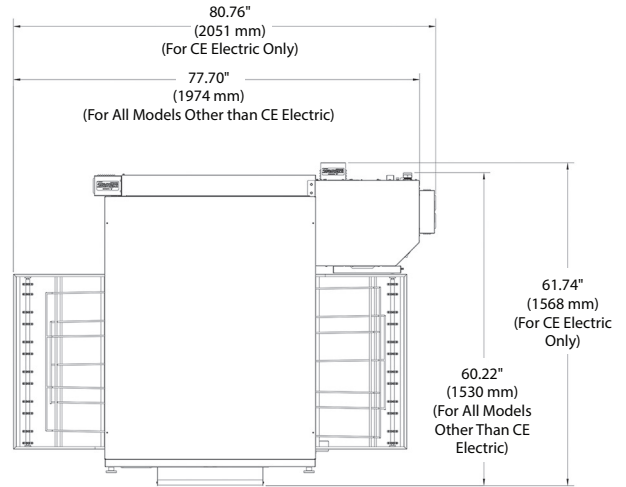
3240 Top View, All Stacking Configurations
