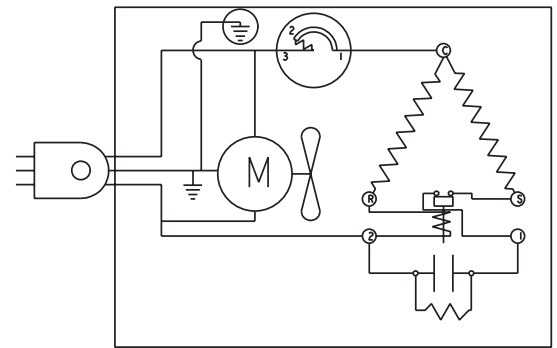
COMPRESSOR
