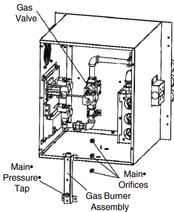
Figure 2-20. Burner Assembly
