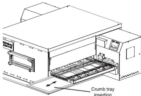
Figure 2-15. Crumb Trays
