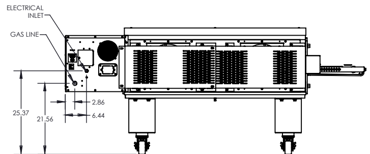
X55 Back View – Gas, 10" Legs Single Unit
