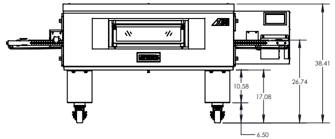
X55 Front View – Gas, 10" Legs Single Unit
