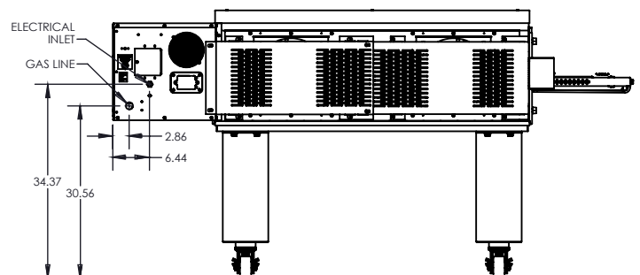
X55 Back View – Gas, 19" Legs Single Unit
