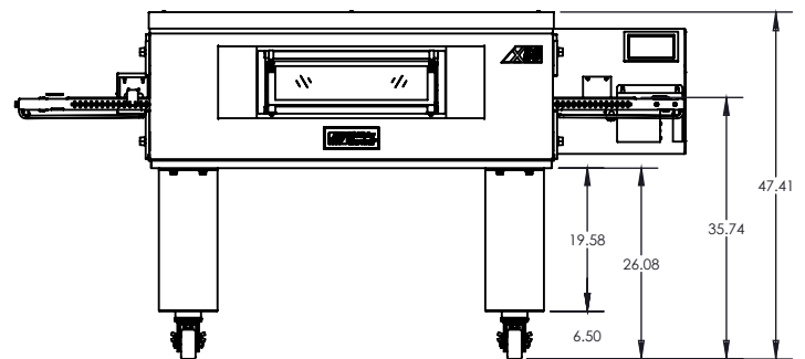
X55 Front View – Gas, 19" Legs Single Unit
