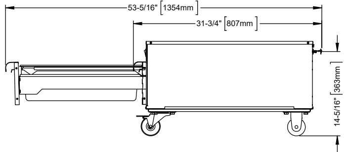
Shown with 3" [76mm] casters
