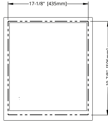
CUT-OUT DIMENSIONS
