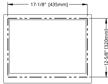
CUT-OUT DIMENSIONS
