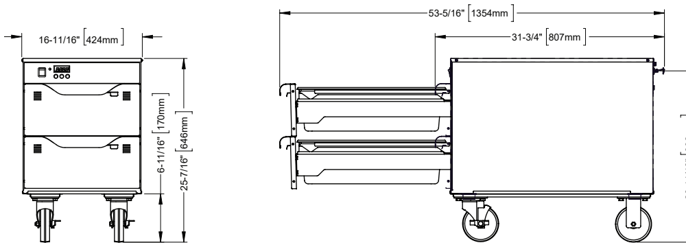
Shown with 5" [127mm] casters
