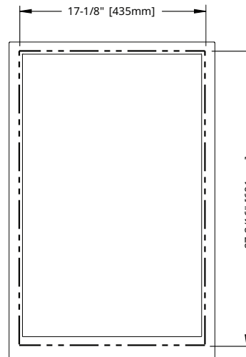
CUT-OUT DIMENSIONS
