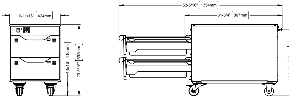
Shown with 3" [76mm] casters
