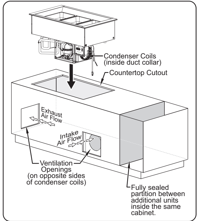
Installing a CWBP-3 Model in a Closed Cabinet
